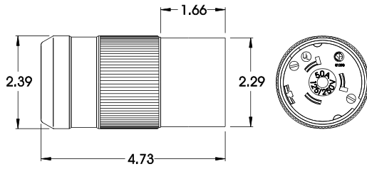
Plug
