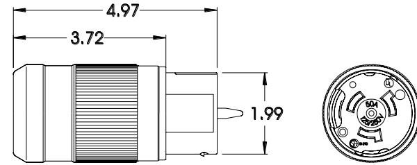
Connector
